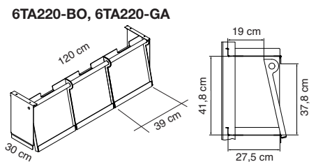
Detail of the magazine rack
